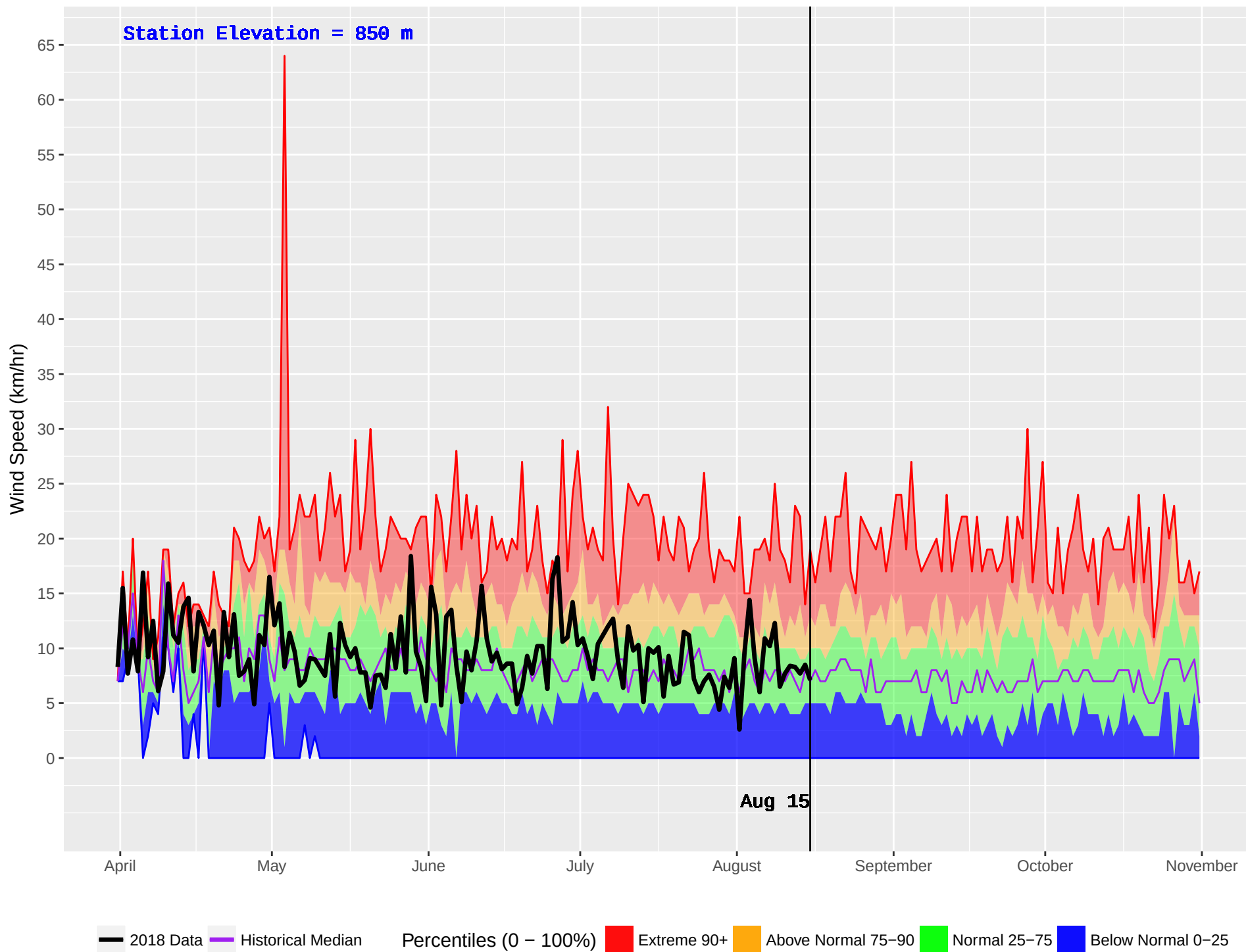
NORTH CHILCO (159) : Historical (1972–2016) and Current (2018) Daily Wind Speed
