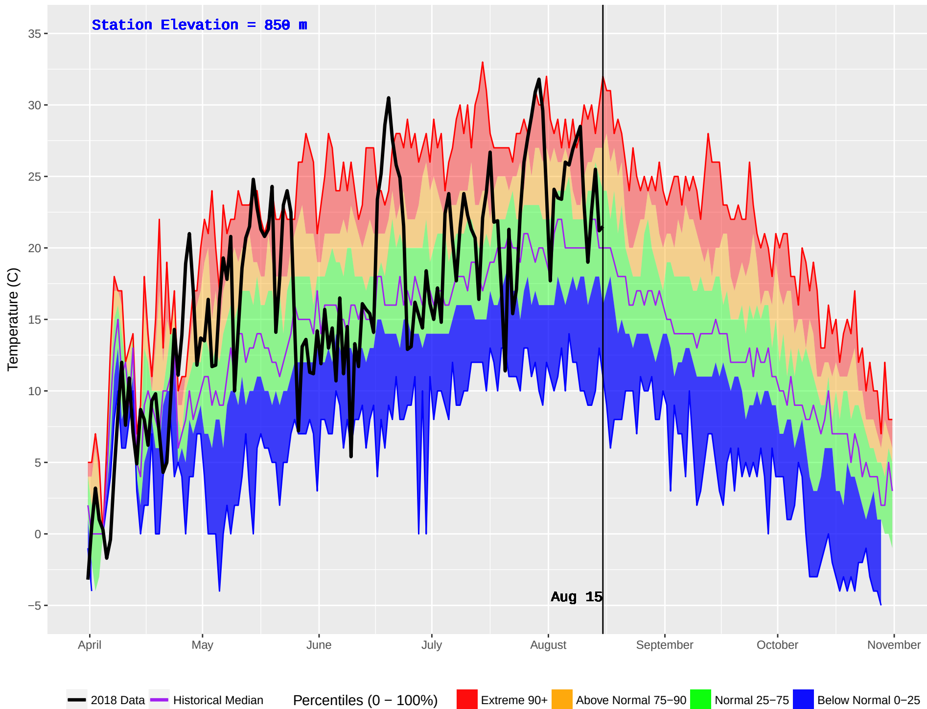
NORTH CHILCO (159) : Historical (1972–2016) and Current (2018) Daily Temperature
