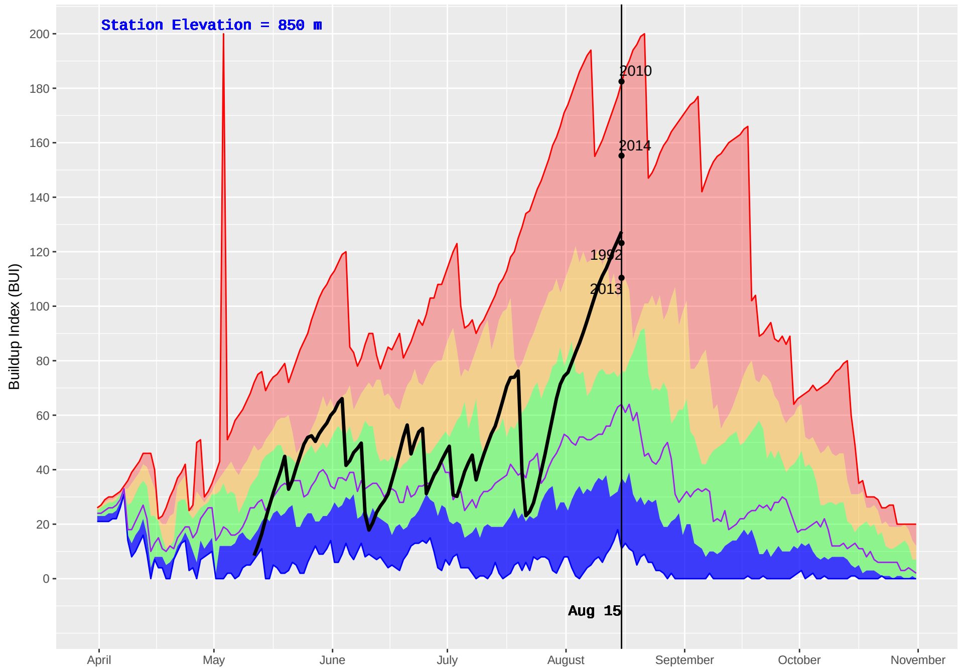
NORTH CHILCO (159) : Historical (1972–2016) and Current (2018) Daily Buildup Index (BUI)
