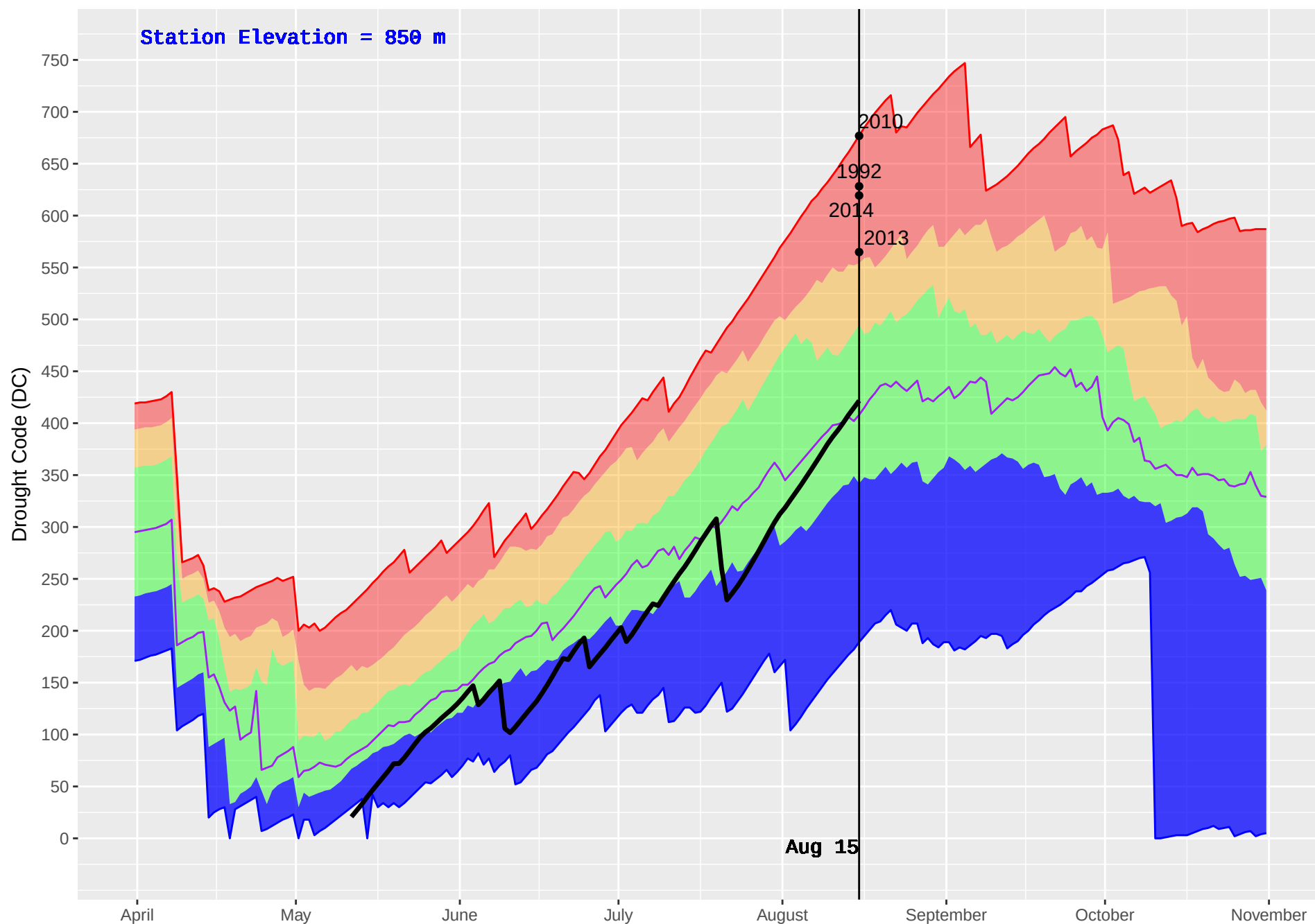
NORTH CHILCO (159) : Historical (1972–2016) and Current (2018) Daily Drought Code (DC)
