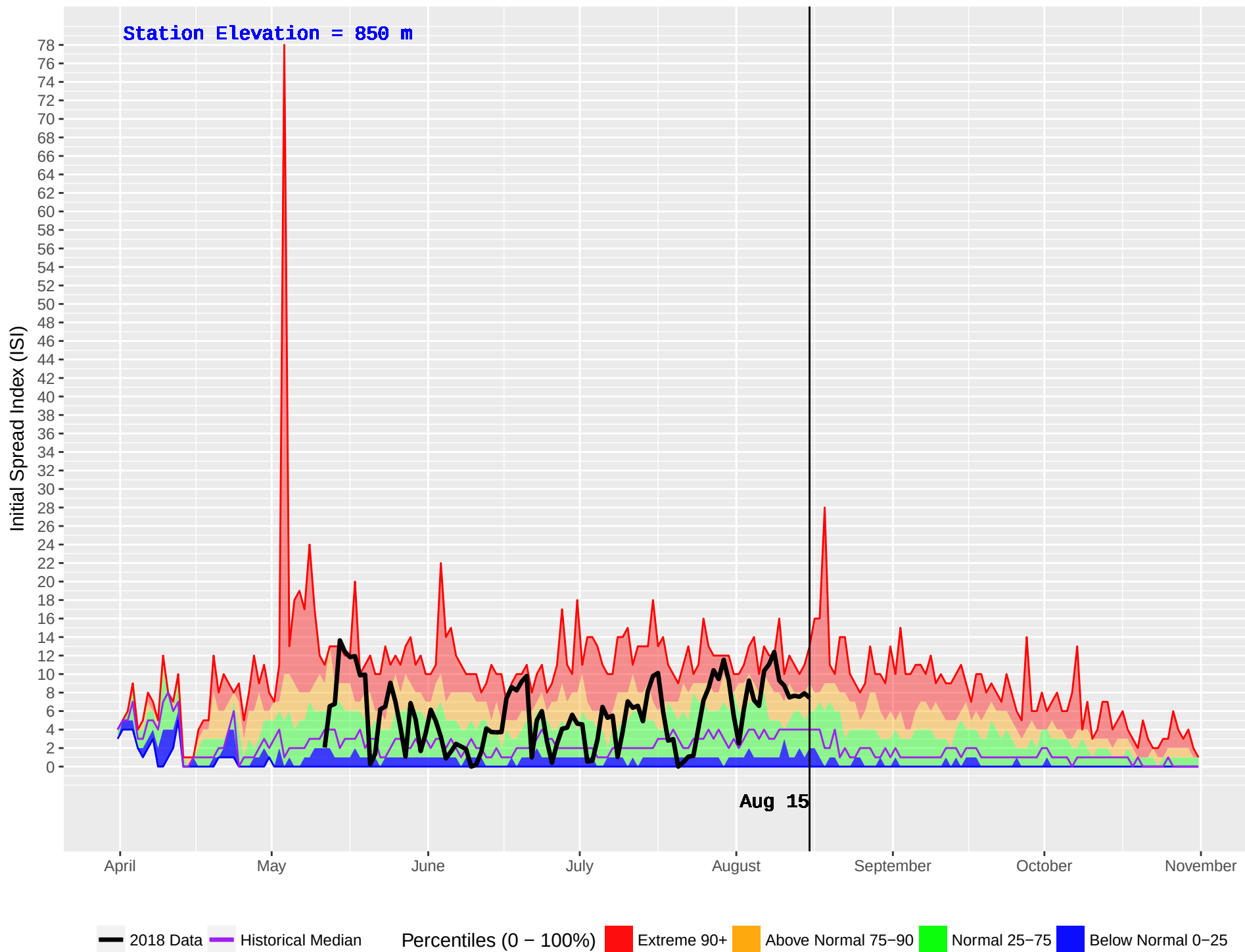
NORTH CHILCO (159) : Historical (1972–2016) and Current (2018) Daily Initial Spread Index (ISI)
